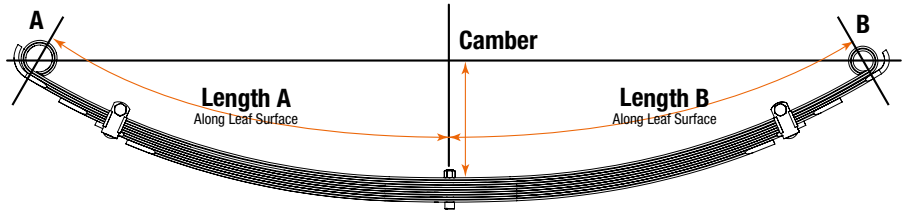
SINGLE STAGE SPRINGS
