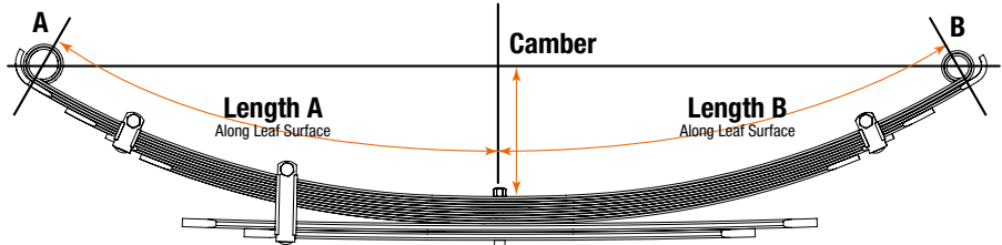
TWO STAGE SPRINGS
