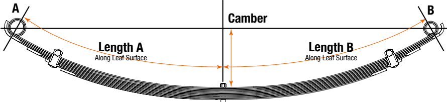
SINGLE STAGE SPRINGS
