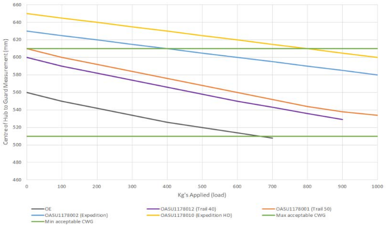
Toyota Landcruiser 78 Series Leaf Spring Deflection
