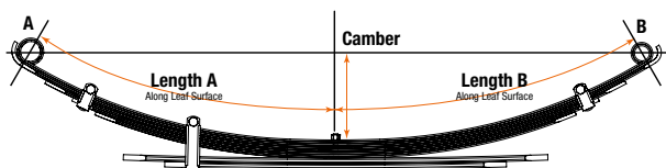
TWO STAGE SPRINGS
